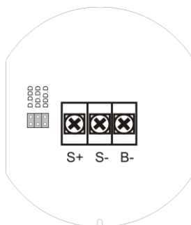
Figure 1. PD6770 Connectors
