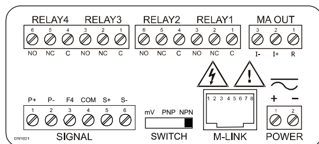
PD6310 Connections
