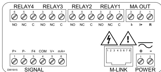
PD6210 Connections
