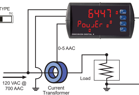
Voltage/Current Input Application Example
