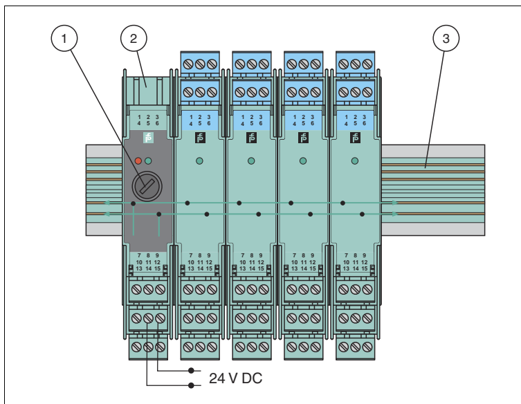
Figure 3.6 Power Rail installation
