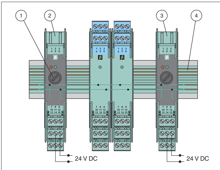
Figure 3.7 Redundant power connections
